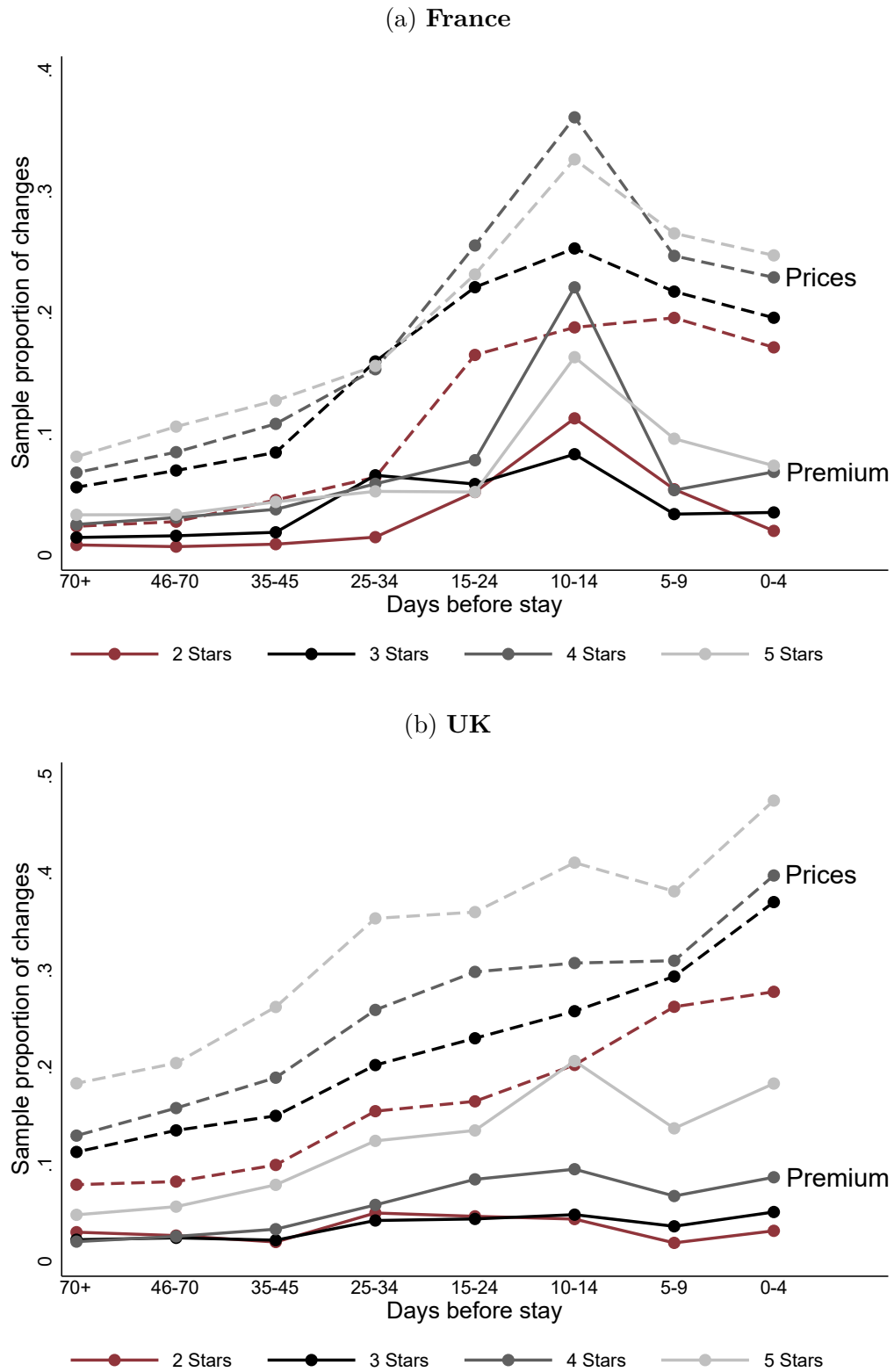
Figure 5: Fraction of rooms experiencing changes in prices and cancellation premia at different lags before stay.
